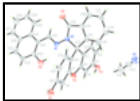
Fig. 1. The asymmetric unit, with the atom-numbering scheme. Displacement ellipsoids are drawn at the 30% probability level.
